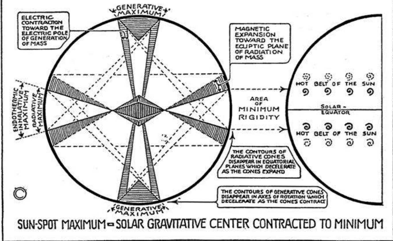
CHART No. 1. THE BREATHING OF THE SUN. EXPLAINING THE PERIODIC SHIFTING OF SUN-SPOTS IN CONFORMITY WITH THE CHANGING MAGNETIC BASES AND ECLIPTIC PLANE OF THE SUN
