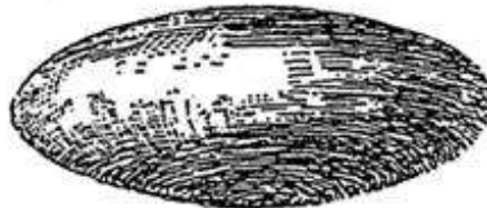
OBLATENESS 3+ DECREASES
