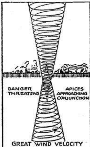
GREAT WIND VELOCITY The apices of contracting cones draw toward each other. The gravitative center contracts to a point of north.
